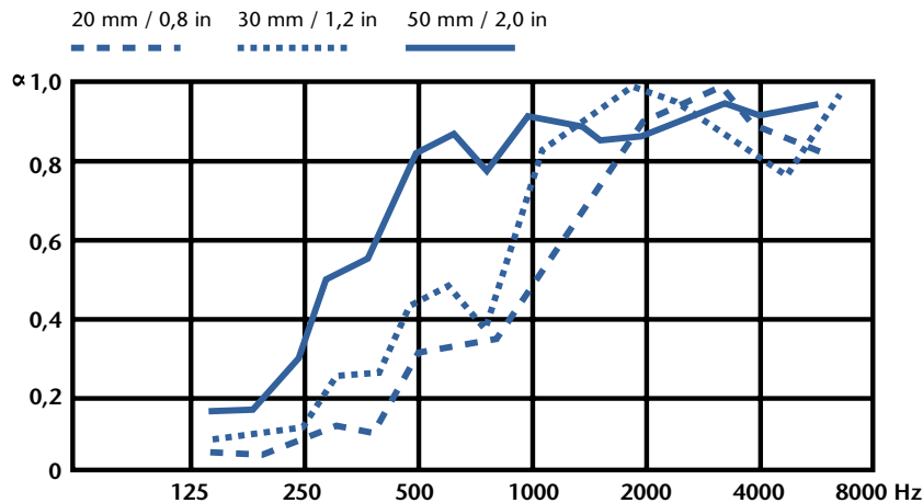
Sound absorption diagram According to DIN 52215
